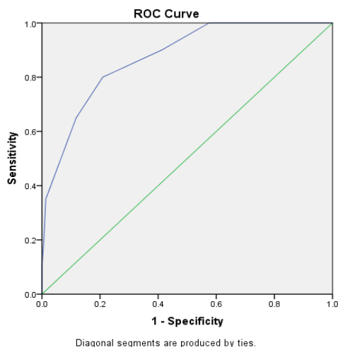
Figure 2: Mortality ROC
